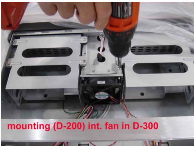
Mounting Front Fan into D-300 Chassis
