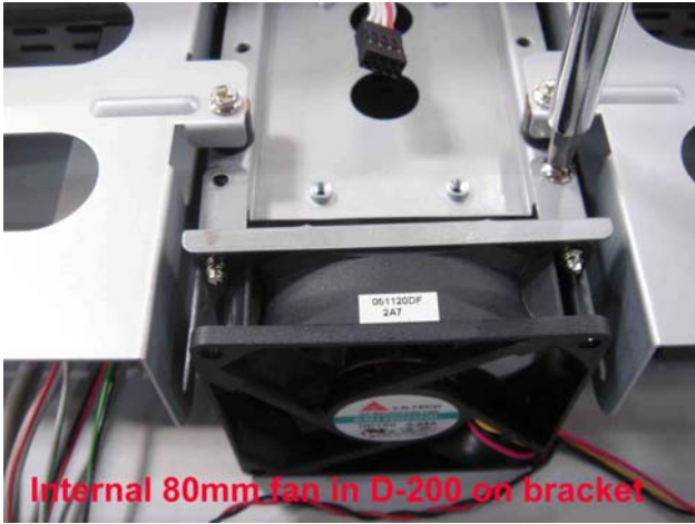
Internal Front Fan in D-200 Chassis
